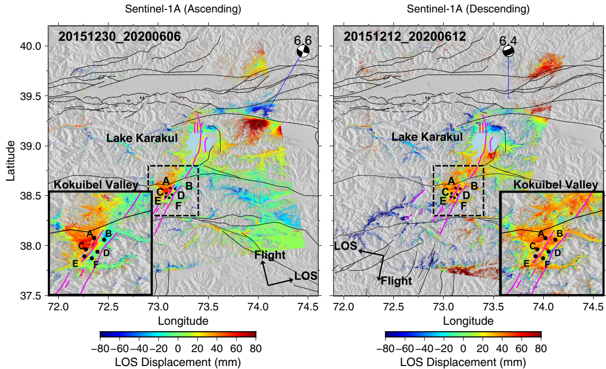
Figure 5. Cumulative Sentinel-1 LOS displacements spanning ~5 years following the mainshock from (a) ascending track 100, and (b) descending track 5. Positive LOS displacements correspond to surface motion toward the satellite. Observation periods are indicated in the top left corner of each panel. The time series of LOS displacements between pair of points “A–B”, “C–D” and “E–F” are shown in Figure 6. Magenta lines denote the SKFS faults. (Insets) Close-up views of postseismic LOS displacements in the Kokuibel Valley area outlined by the dashed rectangle.
