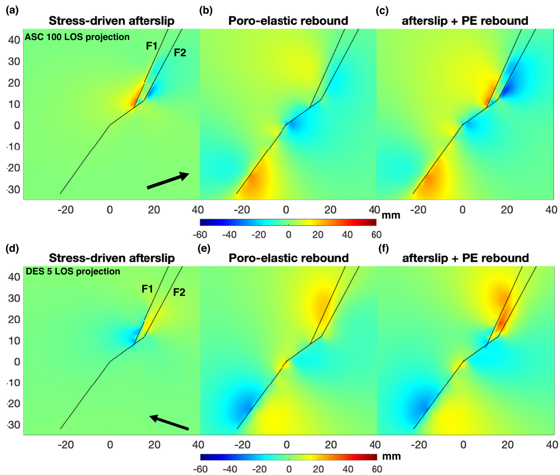
Figure 10. Surface LOS displacements predicted by (a, d) stress-driven afterslip, (b, e) complete poroelastic relaxation and (c, f) a combination of both mechanisms. Other notation is the same as in Figure 8.
