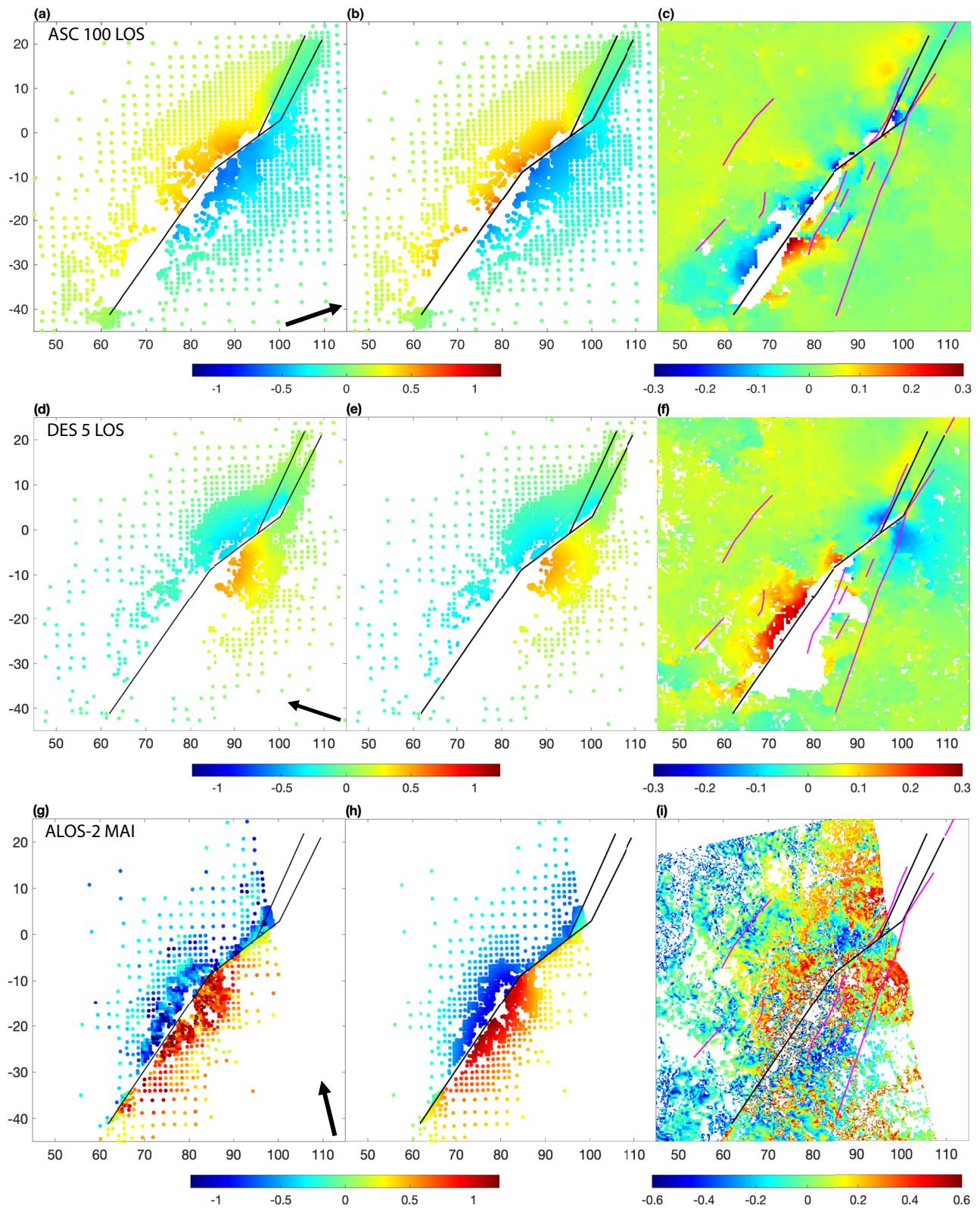
Figure 4. Coseismic (a, d, g) sub-sampled data, (b, e, h) best-fitting models, and (c, f, i) residuals for the Sentinel-1 LOS displacement data from ascending track 100 (top row), descending track 5 (middle row), and ALOS-2 along-track interferogram (bottom row). Color denotes the amplitude of LOS or along-track displacements, in meters. Black arrows show the projection directions. Magenta lines denote the SKFS faults, and black lines denote the modeled trace of the 2015 rupture. Horizontal and vertical axes are in UTM coordinates (easting and northings, respectively) in kilometers, with respect to a local origin (72°E, 38.5°N).
