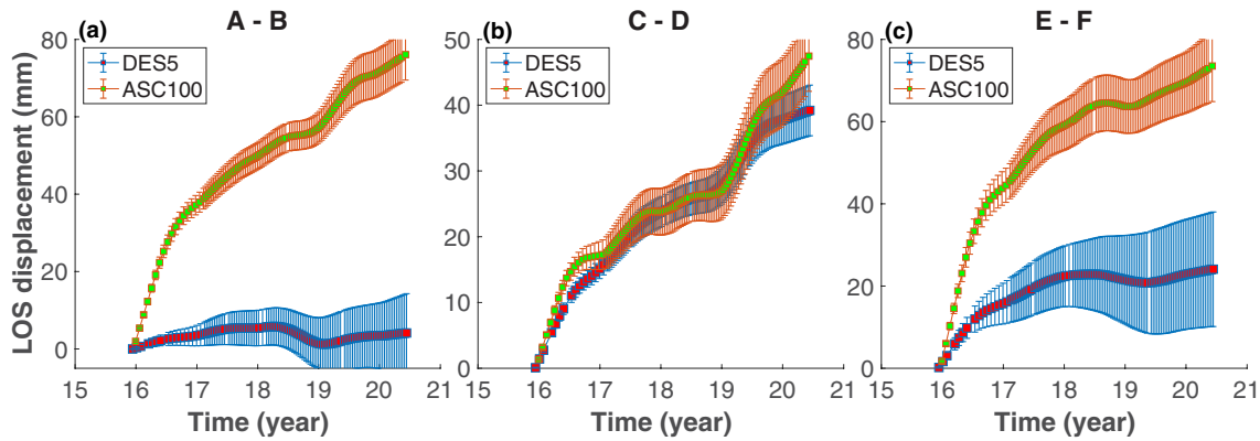
Figure 6. Line of Sight (LOS) displacement time series of relative displacements between the closely-spaced pairs of points (a) A–B, (b) C–D, and (c) E–F spanning the fault trace (see Figure 5). Red dots denote the LOS displacements from the descending track, and green dots denote the LOS displacements from the ascending track. Error bars represent the standard deviation of LOS displacements for persistent scatters within 500 m from the reference points.
