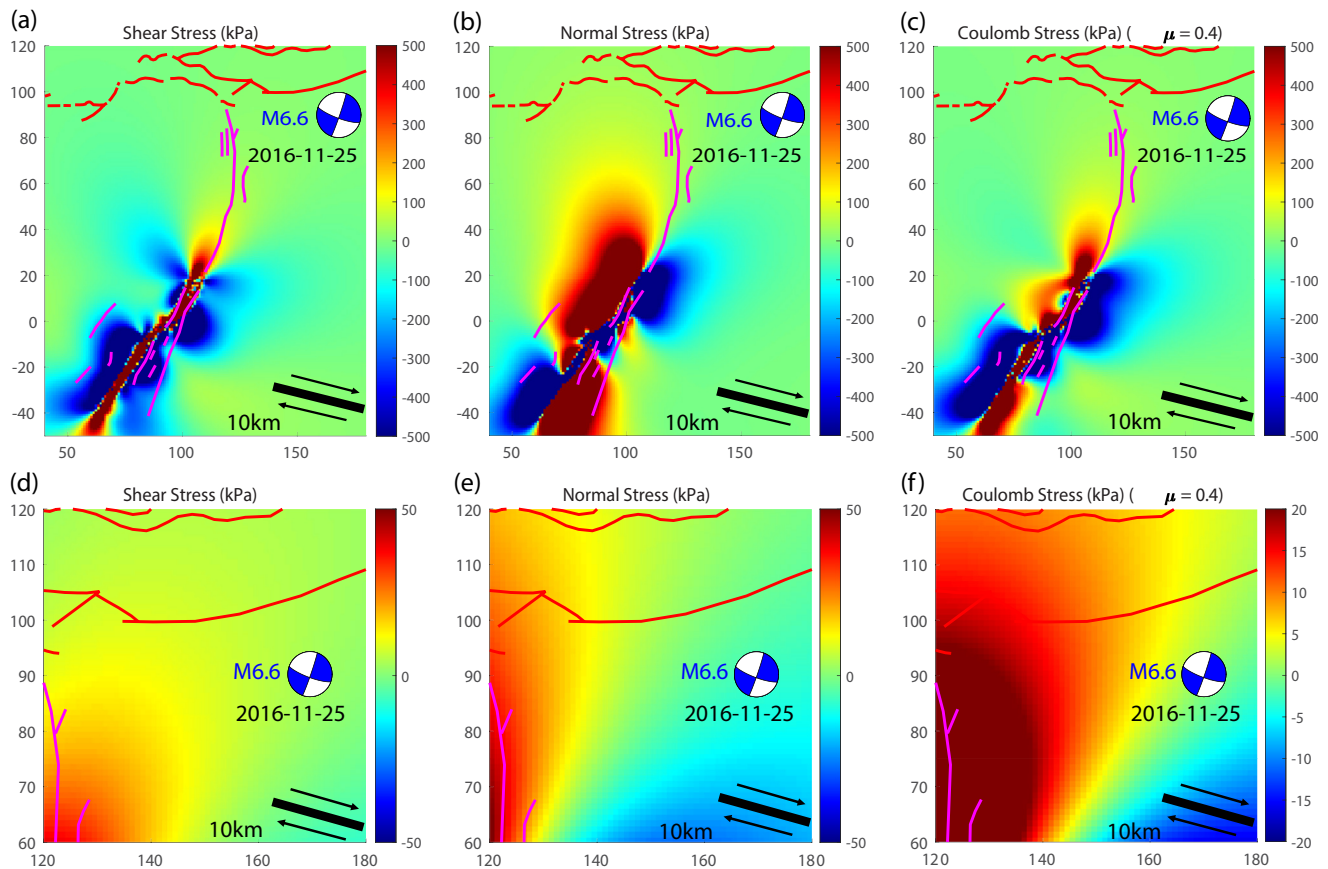
Figure 13. Static stress changes, in kilopascals, due to the M7.2 earthquake at the hypocenter of the 25 November 2016 M6.6 event. Stress changes are computed at depth of 10 km, assuming the average strike of the M6.6 rupture of 107^\circ . Other notation is the same as in Figure 12.
