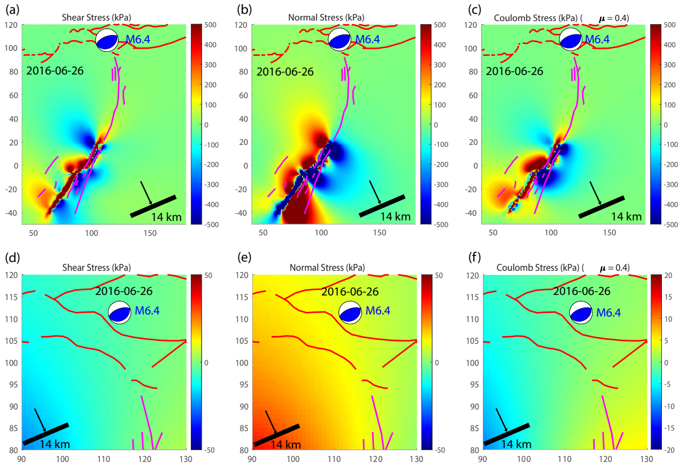
Figure 12. Static stress changes, in kilopascals, due to the M7.2 earthquake at the hypocenter of the 26 June 2016 M6.4 event. Stress changes are computed at the hypocenter depth of 14 km, assuming the average strike of the M6.4 rupture of 248^\circ , and the coefficient of friction of 0.4. (a–c) A regional map. (d–e) A close-up map.
