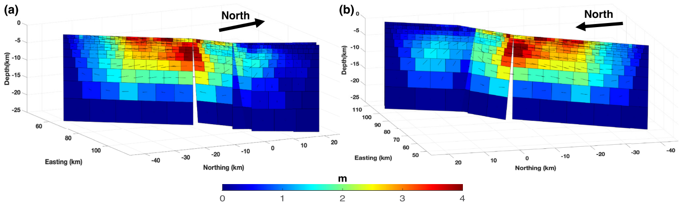
Figure 3. Slip distribution from the joint inversion of space geodetic data assuming a layered elastic-half space model. Colors denote the total amplitude of slip, and arrows show the direction of slip. The two panels (a, b) represent perspectives from different vantage points.
