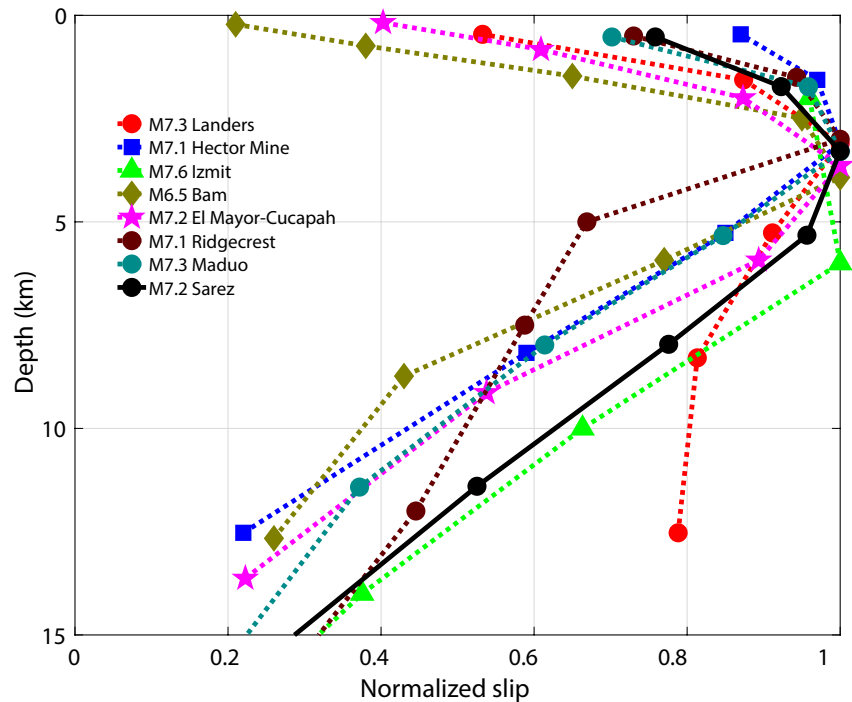
Figure 14. Along-strike averaged coseismic slip as a function of depth for the M 7.2 Sarez (Pamir) earthquake (black solid line), as well as for several other M ~ 7 strike-slip earthquakes (color dashed lines, data from Fialko et al. (2005); Jin and Fialko (2020, 2021); Kaneko and Fialko (2011)).
