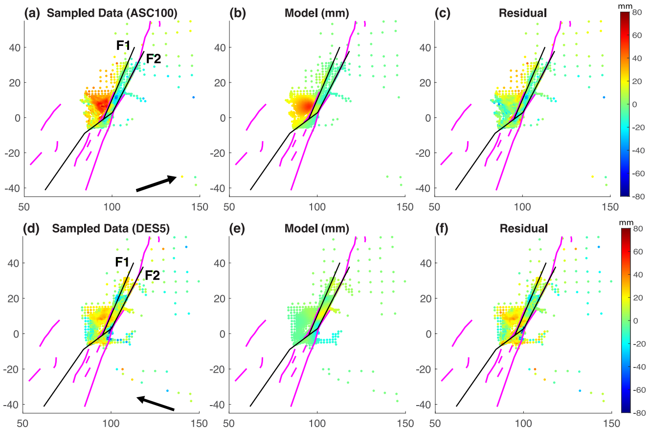
Figure 8. (a, d) Resampled postseismic cumulative surface displacements, (b, e) kinematic model predictions, and (c, f) residuals for the Sentinel-1 ascending track 100 (top row) and descending track 5 (bottom row). Color denotes the amplitude of LOS displacements in millimeters. Black arrows denote the look vectors. Other notation is the same as in Figure 7.
