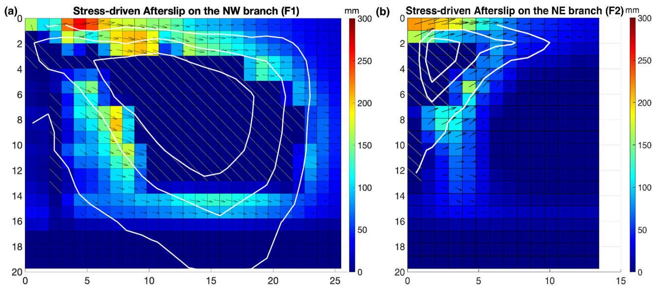
Figure 9. Cumulative afterslip from stress-driven afterslip simulations assuming a rate-strengthening fault friction. Gray hatching denotes fault patches that experienced a coseismic decrease in the Coulomb stress. (a) Afterslip distribution on the F1 segment. (b) Afterslip distribution on the F2 segment (see Figure 7). Colors denote the amplitude of slip, in millimeters. Arrows denote slip direction for each slip patch. White contours denote the coseismic slip (see Figure 3) at 0.5 m intervals, starting at 0.5 m.
